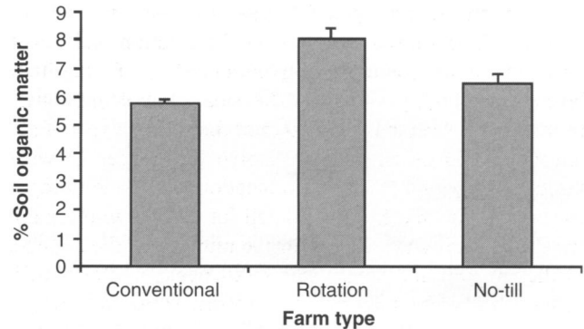
Figure 2. Percent soil organic matter by weight in conventional, rotation and no-till agroecosystems. Organic matter was calculated from soil cores 25 cm deep. Means \pm standard error are shown. ( N = 6 , P = 0.0034 ).
