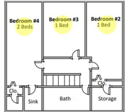
2nd Level Floor Plan
